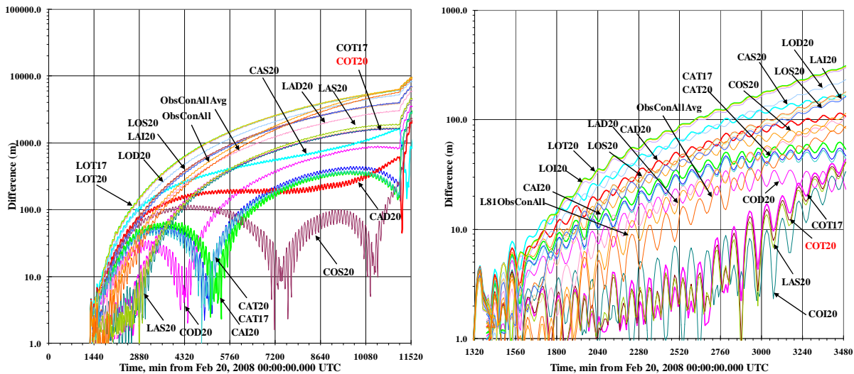
Figure 14: Sample Atmospheric Drag Sensitivity: Positional differences are shown for ICESat (satellite 27642) using various data approaches with the NRLMSISE-00 model. The POE comparison was used to evaluate each atmospheric model. Note that each of the atmospheric models used a daily interpolation on the geomagnetic indices. The same initial conditions were used for each run, but the axes scales are different.
