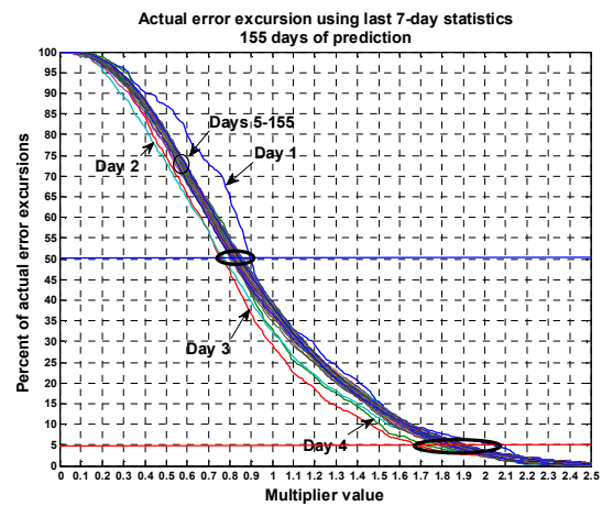
Figure 21 – Multiplier analysis for actual error excursions using last 7 day error statistics
