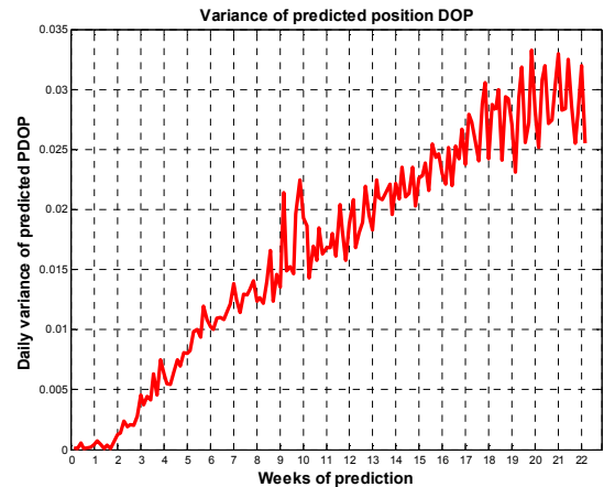
Figure 6 - Variance of Predicted Position DOP
