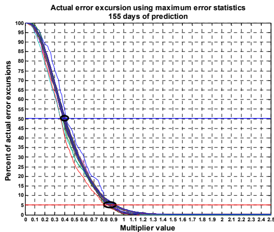
Figure 22 - Multiplier analysis for actual error excursions using maximum error statistics
