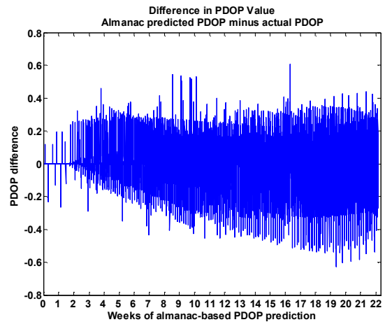
Figure 1 - PDOP Residuals 22 Weeks
