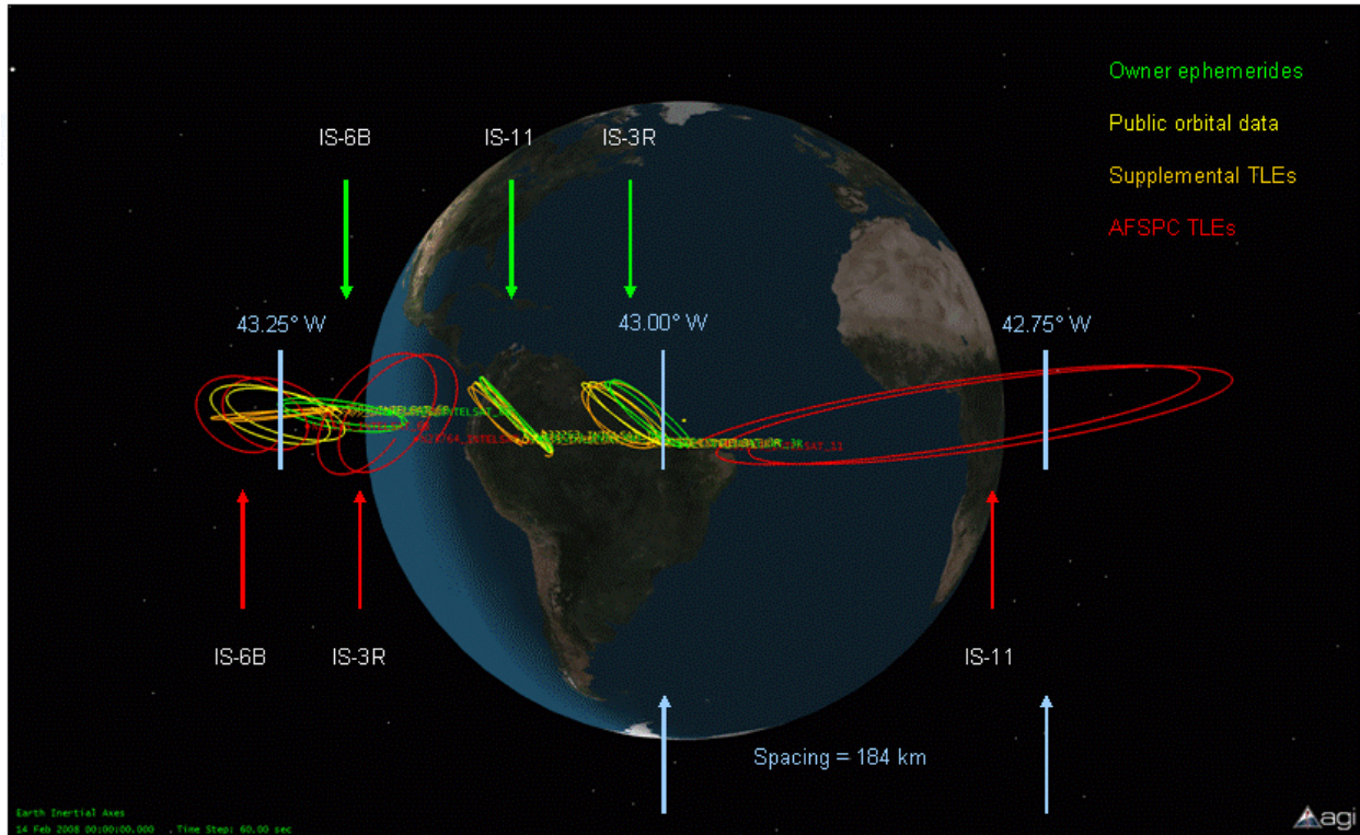
Fig. 4. Comparison of Orbital Products for Intelsat 3R, 6B, and 11
