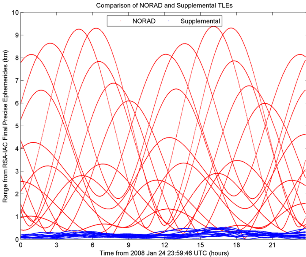
Fig. 3. Comparison of NORAD and Supplemental TLEs for GLONASS
