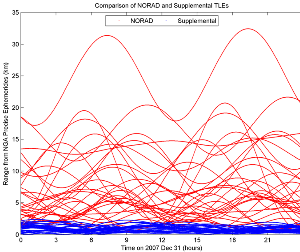
Fig. 2. Comparison of NORAD and Supplemental TLEs for GPS
