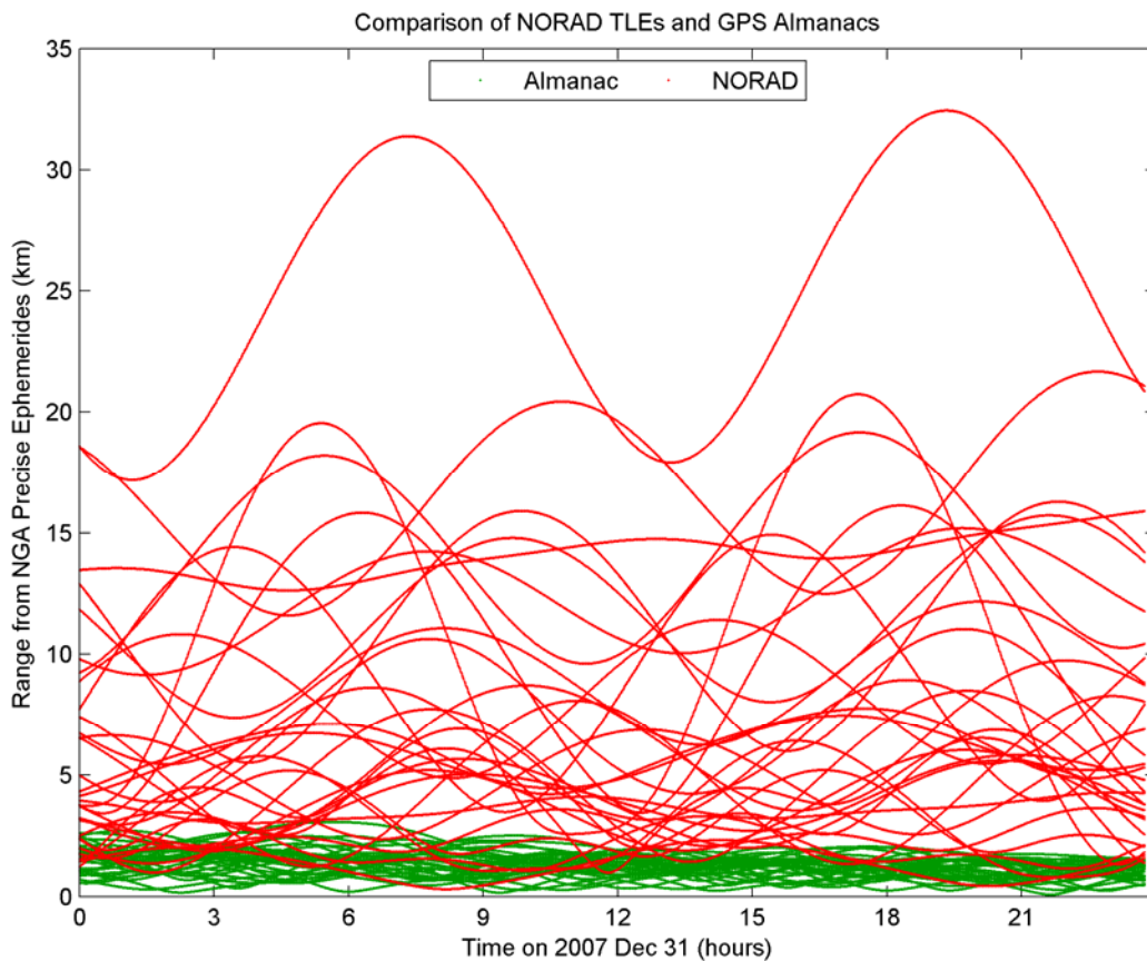
Fig. 1. Comparison of NORAD TLEs and GPS Almanacs
