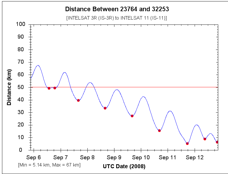
Fig. 6. Neighborhood Watch Plot
