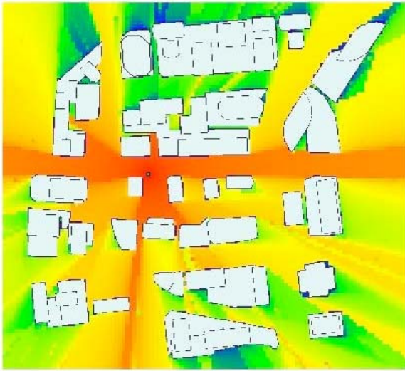
Figure 5. (U) Real Time Path Loss, Rosslyn, VA
