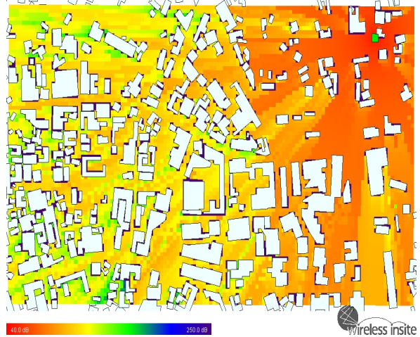
Figure 9. (U) Real Time Path Loss, Ramadi, Iraq The small square represents the transmitter.
