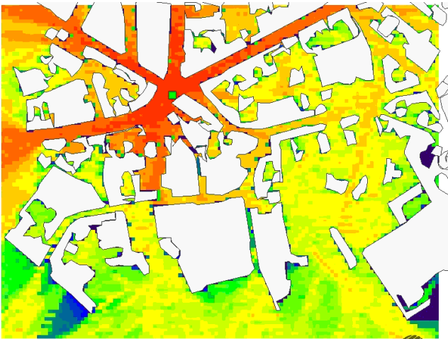
Figure 6. (U) Full 3D Path Loss, Milan, Italy
