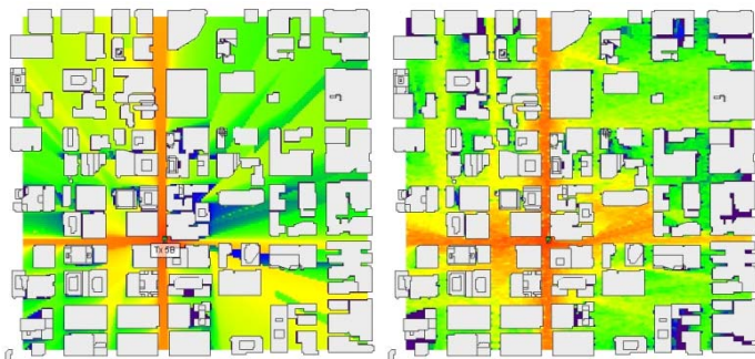
Figure 3. (U) Comparison of Wireless InSite Full 3D (left) and Real Time (right) in Chicago
