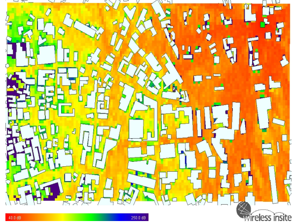
Figure 8. (U) Full 3D Path Loss, Ramadi, Iraq
