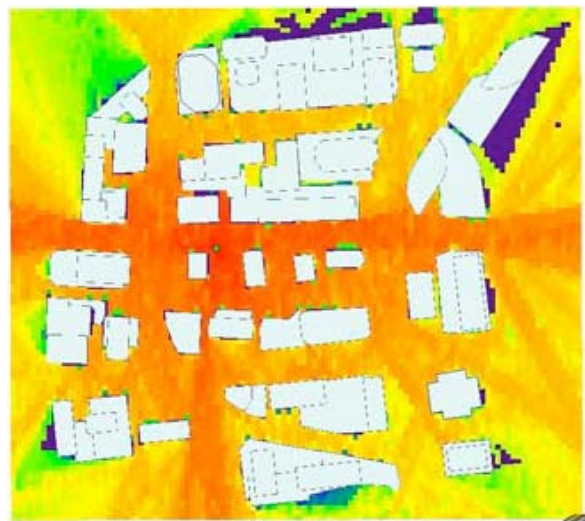
Figure 4. (U) Full 3D Path Loss, Rosslyn, VA
