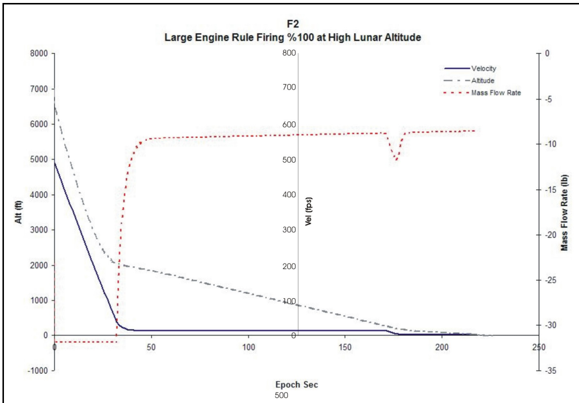
Figure 21: Simulation F2 (100% DoS at Higher Altitude)
