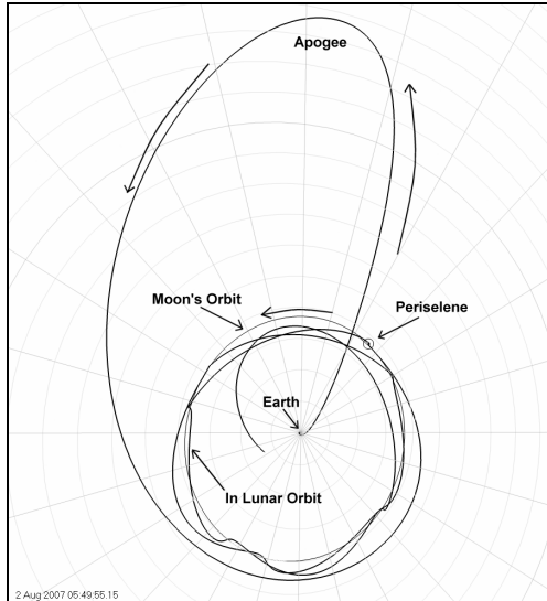
Figure 4: WSB in Earth Inertial Coordinates
