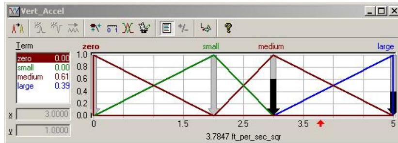
Figure 20: Fuzzy Output Set Vertical Acceleration
