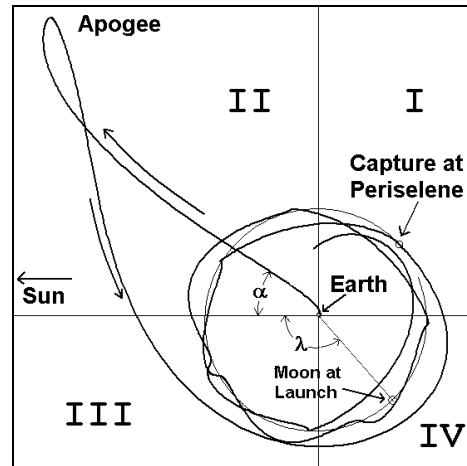
Figure 5: WSB in Sun-Earth Rotating Coordinates
