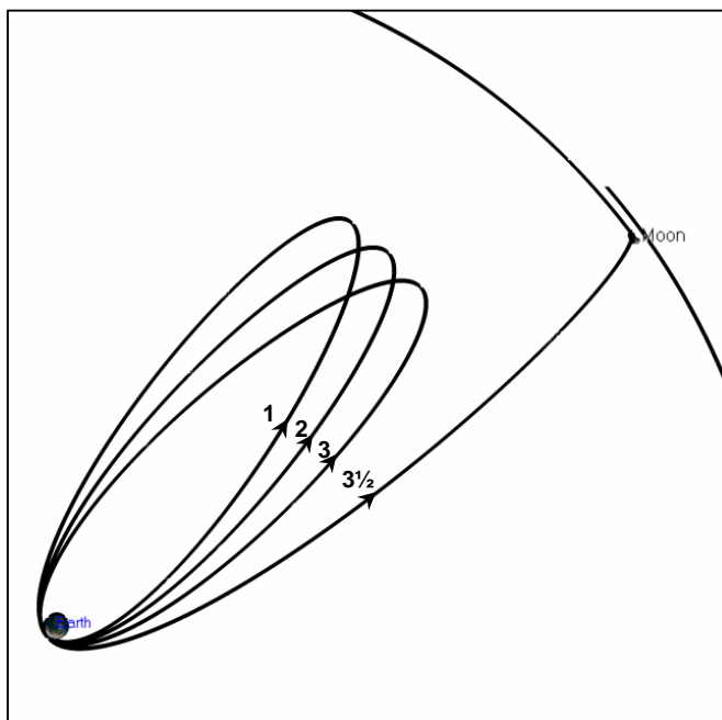
Figure 2: Ballistic Transfers in Earth-Moon Rotating Coordinates
