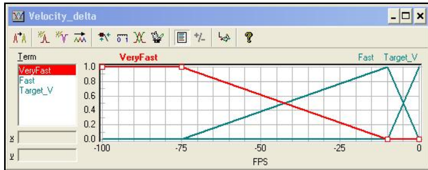
Figure 17: Fuzzy Input Set Velocity \Delta
