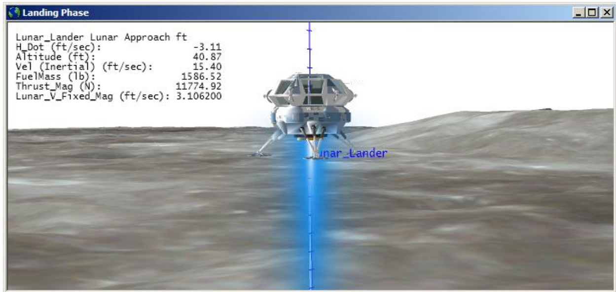
Figure 12: Screen Capture of Ke-V from Landing Numerical Simulation
