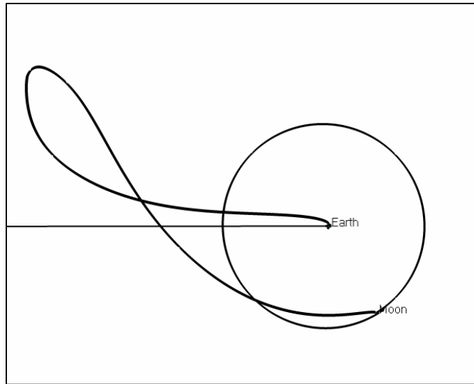
Figure 7: WSB Transfer in Sun-Earth Rotating Coordinates
