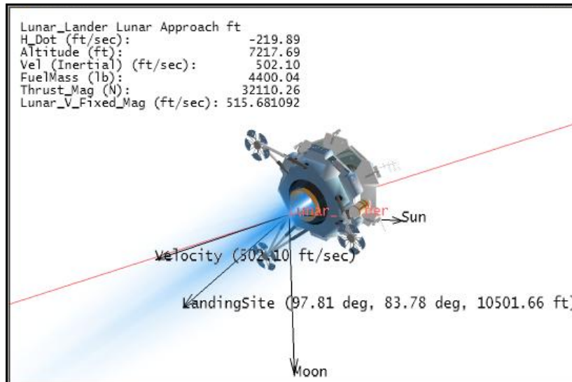
Figure 11: Screen capture of Ke-V during Descent Phase Numerical Simulation
