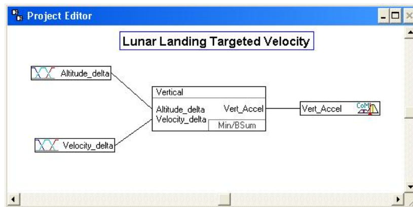
Figure 15: Lunar Landing Fuzzy Logic System
