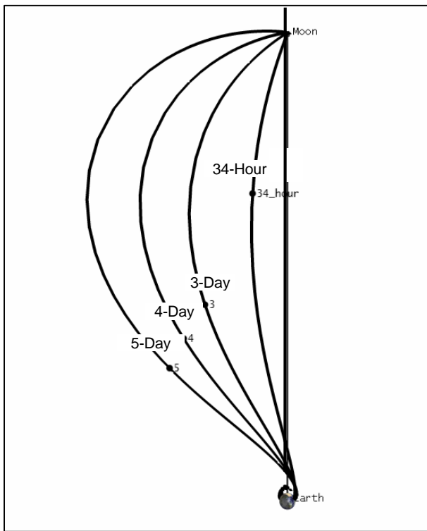
Figure 2: Ballistic Transfers in Earth-Moon Rotating Coordinates
