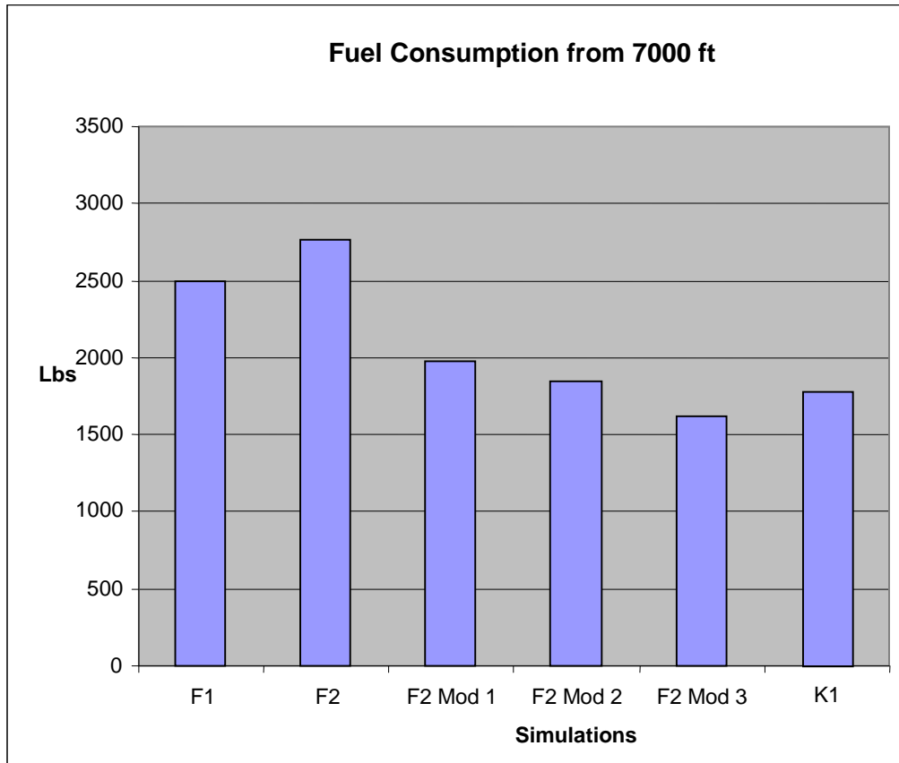
Figure 23: Fuel consumption comparison for Fuzzy Logic F2 Flights from 7000 ft
