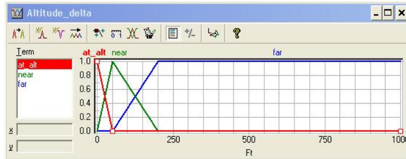
Figure 16: Fuzzy Input Set Altitude \Delta
