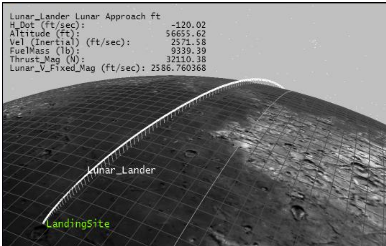
Figure 10: Screen Capture of Braking Phase from Numerical Simulation
