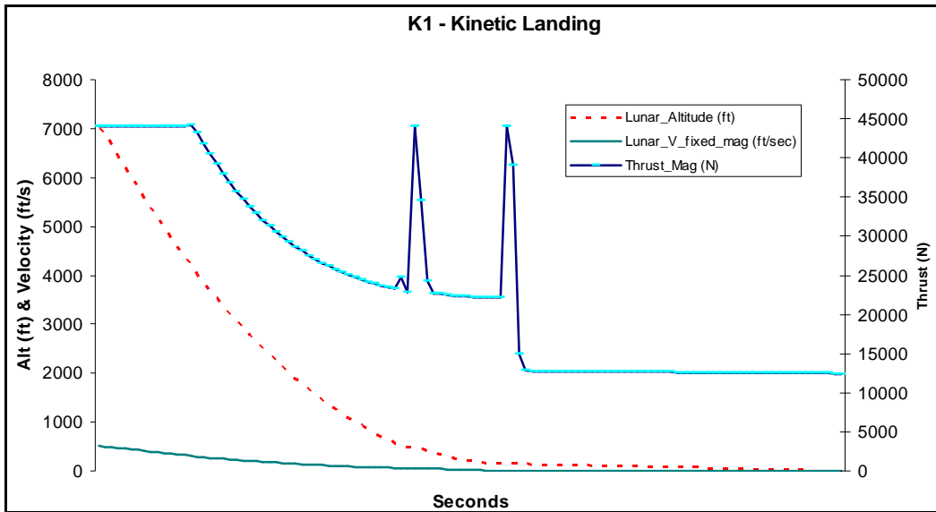
Figure 13: Altitude, Velocity, and Thrust Magnitude
