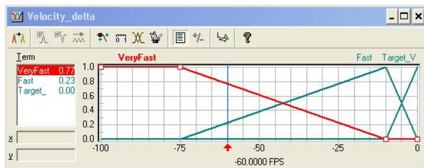
Figure 18: Fuzzy Input Set Velocity \Delta for -60 ft/s from STK Simulation
