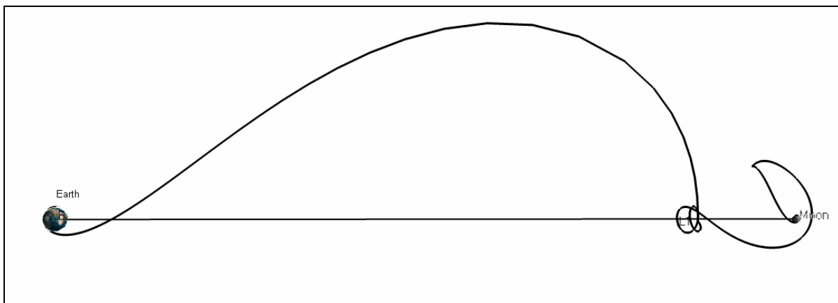
Figure 8: Earth to L1 to Lunar Landing in Earth-Moon Rotating Coordinates
