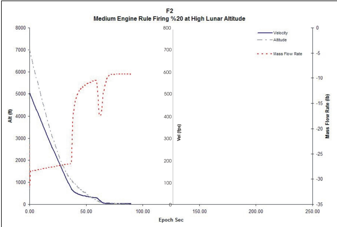
Figure 22: Simulation F2 Mod 3 (20% DoS at Higher Altitude)
