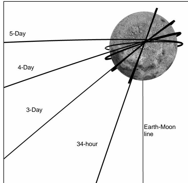
Figure 9: Different relative RAANs vs. Time-of-Flight in Earth-Moon Rotating Coordinates
